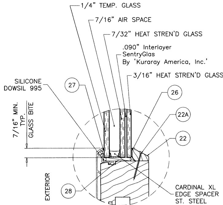
GLAZING DETAIL 1-1/4" OVERALL INSUL. LAM. GLASS
